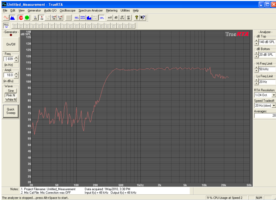
JA6681B on 425 Horn, mic at plane of mouth, 400Hz 18dB HP (no other filters) 1-May-10
