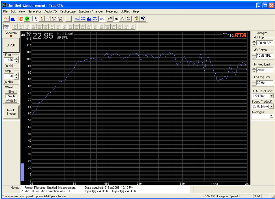
Lower on 2.3m bass horn alone, no filters, mic in horn mouth
