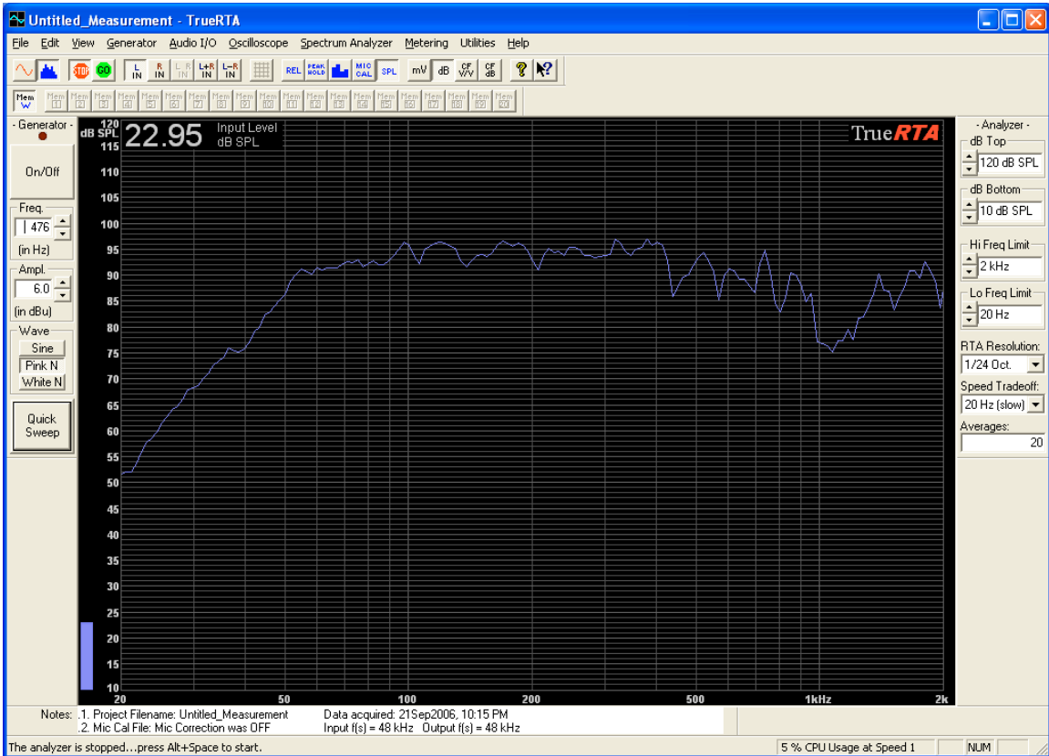
Lower on 2.3m bass horn alone, no filters, mic in horn mouth
