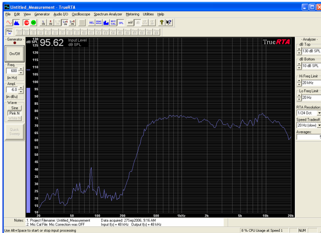
350Hz HP cross over – mic at horn mouth – pink noise
